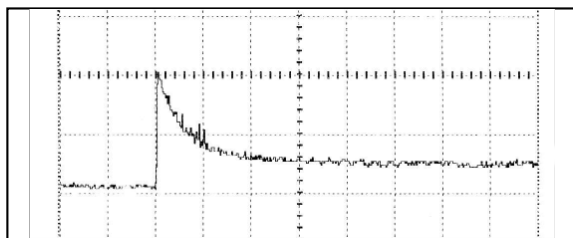
Figure 7. Typical magnetron pulse from an interrupter.
