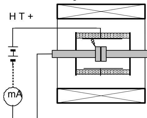
Fig. 6. A schematic Magnetron Circuit.
