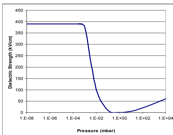
Figure 2: The Paschen Curve, Showing How Breakdown Voltage Varies With Vacuum Pressure. Note that pressure increases to the right, but degree of vacuum increases to the left.
